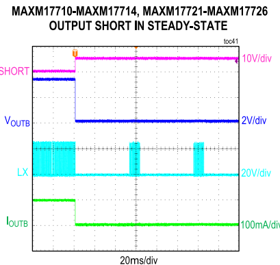
CONDITIONS: PWM MODE, V_{OUTB} = 3.3V , I_{OUTB} = 100mA , I_{OUTL} = 50mA , f_{SW} = 375kHz
