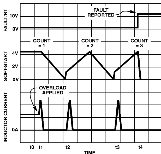
FIGURE 8. OVER-CURRENT OPERATION
