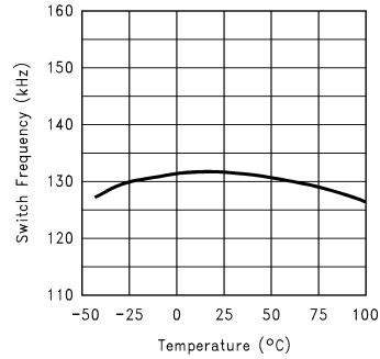
Switch Frequency vs. Temperature ( V_{IN} = 3.6\text{V} )
