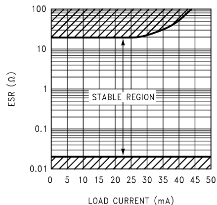
FIGURE 5. ESR Curve for C_{OUT} = 10\mu\text{F}
