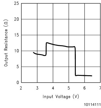
Output Resistance ( V_{DBL} ) vs. Input Voltage
