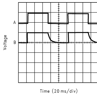
V_{PSW} Response to CE (with 5mA Load)
