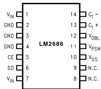
14-Pin TSSOP
