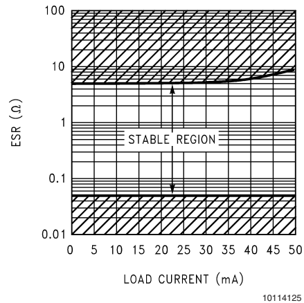
FIGURE 3. ESR Curve for C_{OUT} = 2.2\mu\text{F}
