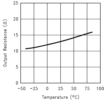
Output Resistance (VDBL) vs. Temperature ( V_{IN} = 3.6\text{V} )
