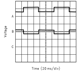
Line Transient Response (with 5mA Load)
