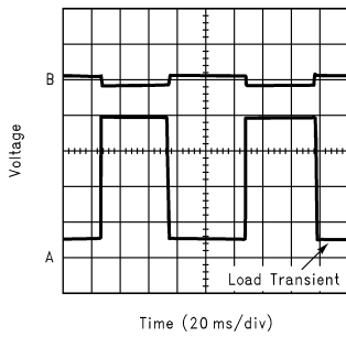
V_{O5} Load Transient Response
