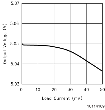
Output Voltage ( V_{O5} ) vs. Load Current ( V_{IN} = 3.6\text{V} )
