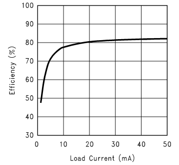
Efficiency vs Load Current ( V_{IN} = 3.0\text{V} )
