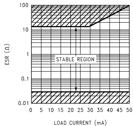
FIGURE 4. ESR Curve for C_{OUT} = 4.7\mu\text{F}
