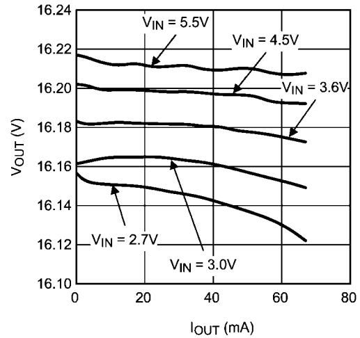
Load Regulation (V OUT = 16 V)
