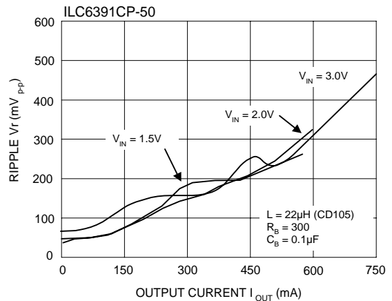
Ripple Voltage vs. Output Current
