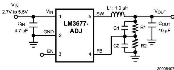
FIGURE 2. Typical Application Circuit - ADJ. Version
