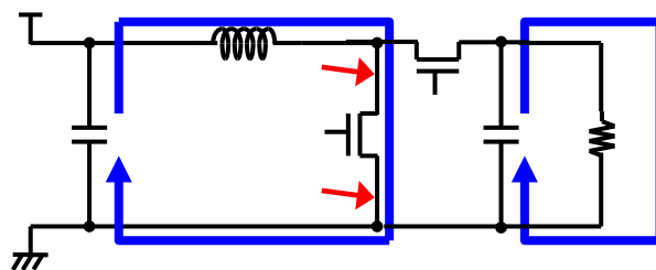
Figure 1. MOSFET-ON
