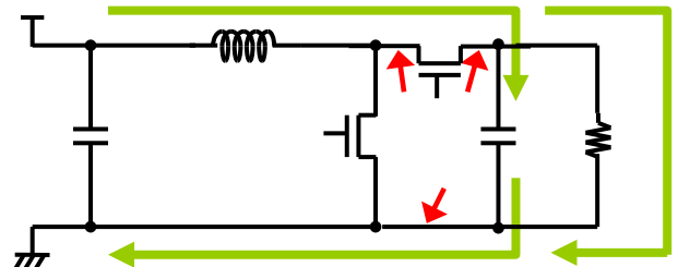
Figure 2. MOSFET-OFF
