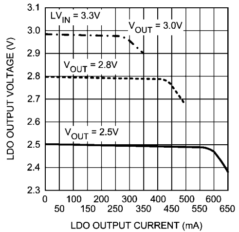
LDO V OUT vs. Load Current
