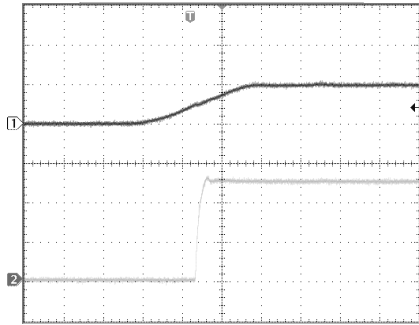
LDO Startup Waveform (LV_IN Fast Rising Edge)
