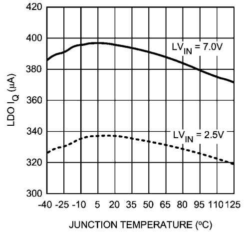
LV IN Quiescent Current vs. Temperature
