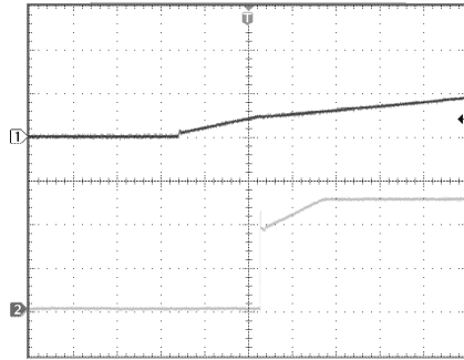
LDO Startup Waveform (LV_IN Slow Rising Edge)
