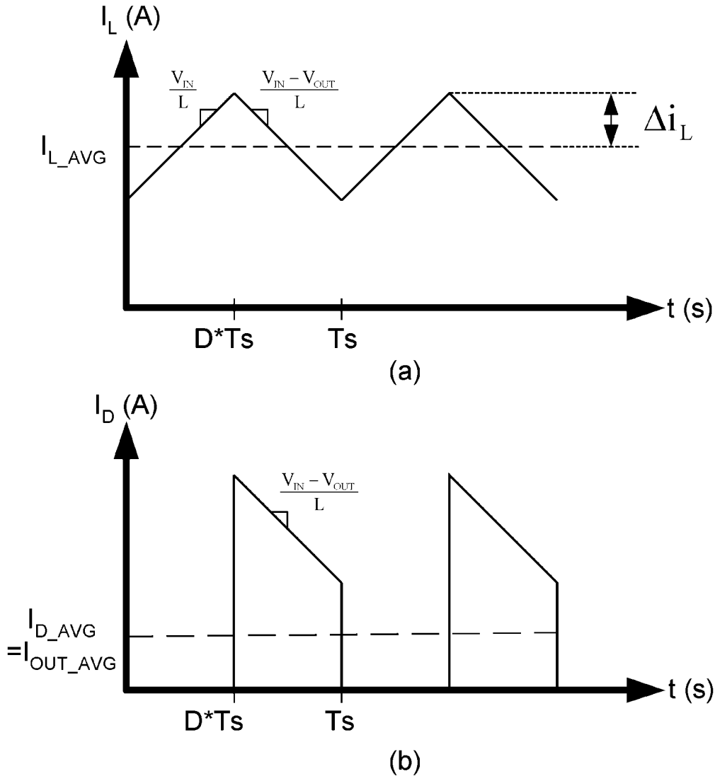
FIGURE 5. (a) Inductor current. (b) Diode current.
