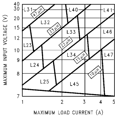
FIGURE 4. LM2677-5.0
