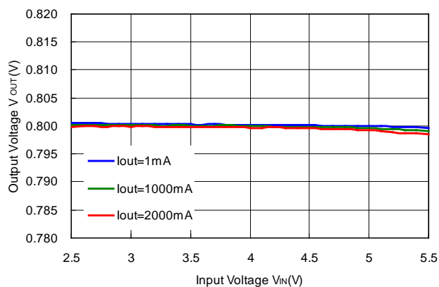
RP506Lxx1K/L/M V_{OUT} = 0.8\text{ V} MODE = "H" Forced PWM Control
