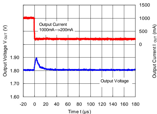
RP506Lxx1K/L/M ( V_{IN} = 3.6\text{ V} , V_{OUT} = 1.8\text{ V} )
