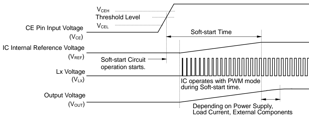
Timing Chart
