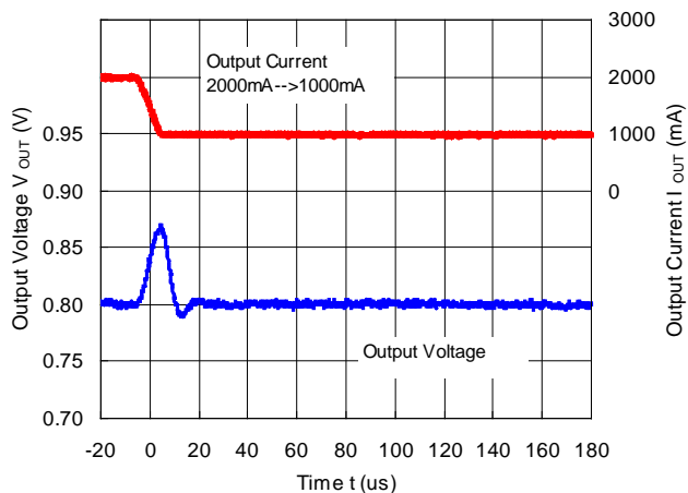
RP506Lxx1K/L/M ( V_{IN} = 3.6\text{ V} , V_{OUT} = 0.8\text{ V} )
