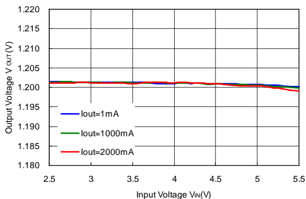
RP506L V_{OUT} = 1.2\text{ V} MODE = "H" Forced PWM Control
