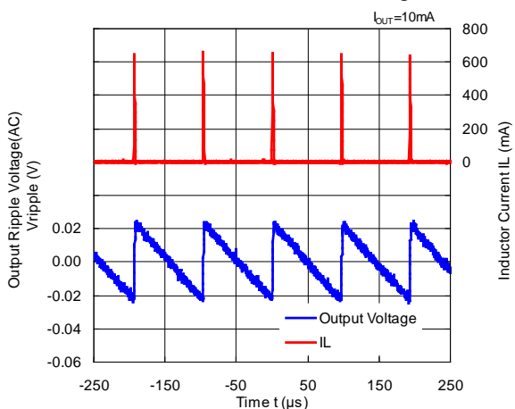
RP506Lxx1K/L/M V_{OUT} = 0.6\text{ V} ( V_{IN} = 3.6\text{ V} ) MODE = "L" PWM/VFM Auto Switching Control
