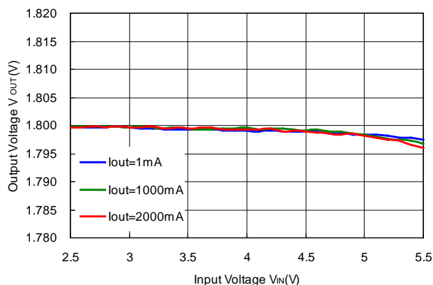
RP506L V_{OUT} = 1.8\text{ V} MODE = "H" Forced PWM Control
