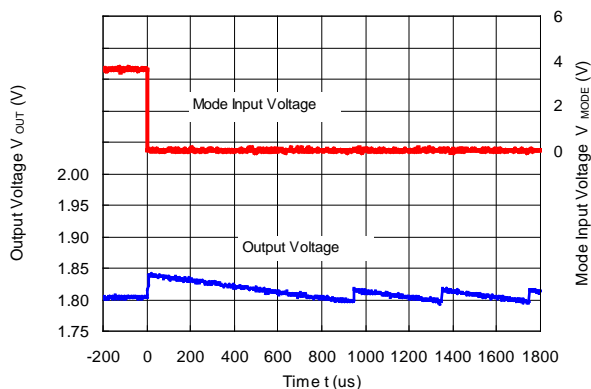
RP506Kxx1D/E/F (V IN = 3.6 V, V OUT = 1.8 V, I OUT = 1 mA) MODE = "H" --> MODE = "L"
