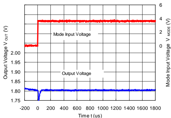
RP506Kxx1D/E/F (V IN = 3.6 V, V OUT = 1.8 V, I OUT = 1 mA) MODE = "L" --> MODE = "H"
