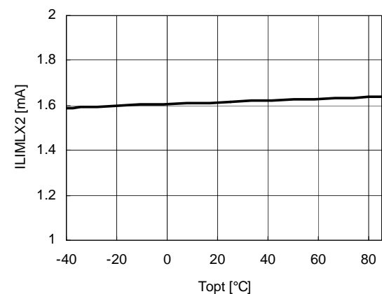
12) LX2 Limit Current vs. Temperature R1283x00xx
