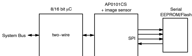
Figure 28. Host Mode with Flash
