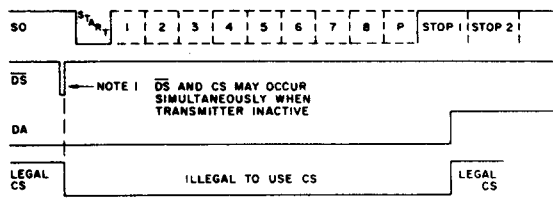
Fig.30 ALLOWABLE POINTS TO USE CONTROL STROBE
