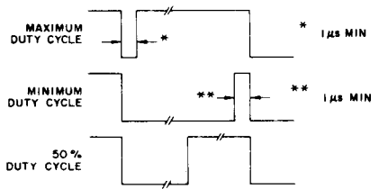
Fig.31 ALLOWABLE TCP, RCP
