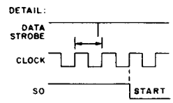
Fig.27 UAR/T — TRANSMITTER TIMING
