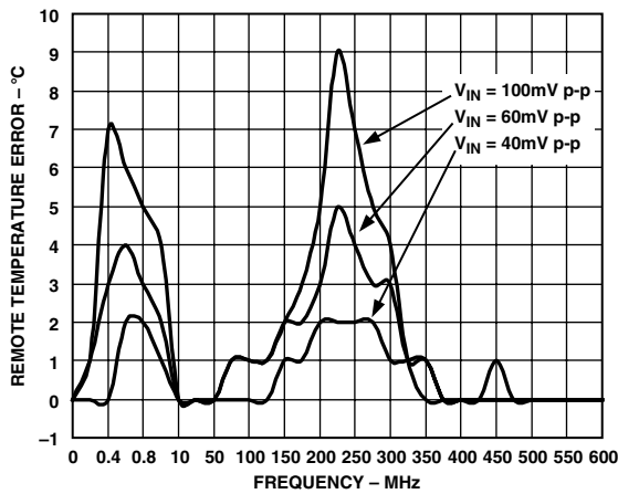
TPC 3. Remote Temperature Error vs. Common-Mode Noise Frequency
