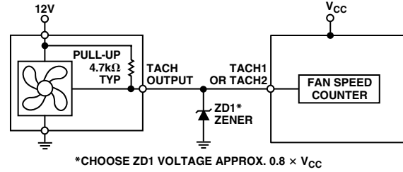
Figure 9b. Fan with Tach. Pull-Up to Voltage >6.5 V (e.g., 12 V) Clamped with Zener Diode
