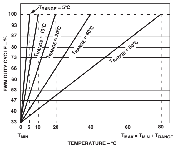
Figure 11. PWM Duty Cycle vs. Temperature Slopes ( T_{RANGE} )
