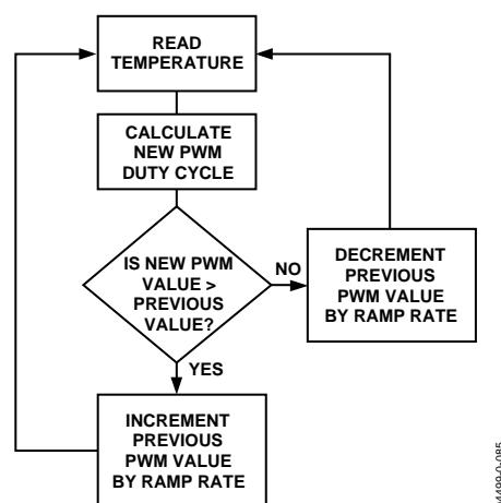
Figure 84. Enhanced Acoustics Algorithm
