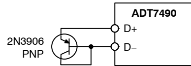
Figure 26. Measuring Temperature by Using a PNP Transistor
