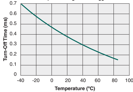
Typical Turn-Off Time vs. Temperature ( I_F=5mA, I_L=170mA_{DC} )
