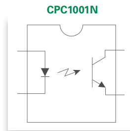
4-Pin SOP
