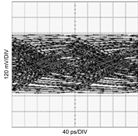
FIGURE 32. Unequaled Signal (10m 24AWG PCIe Cable, 5Gbps, PRBS7)
