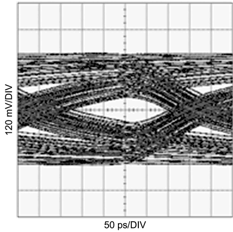
FIGURE 29. Unequaled Signal (10m 24AWG PCIe Cable, 2.5Gbps, PRBS7)
