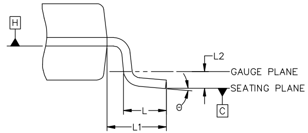
VIEW C
