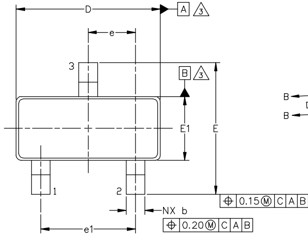
Figure 12. 3-pin SOT23 Package
