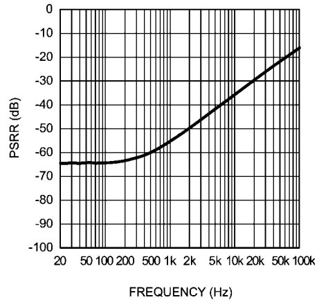
INT/EXT MICBIAS PSRR vs Frequency V_{DD} = 5V , MICBIAS = 2.5V
