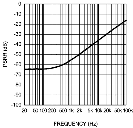
INT/EXT MICBIAS PSRR vs Frequency V_{DD} = 3.3V , MICBIAS = 2.5V
