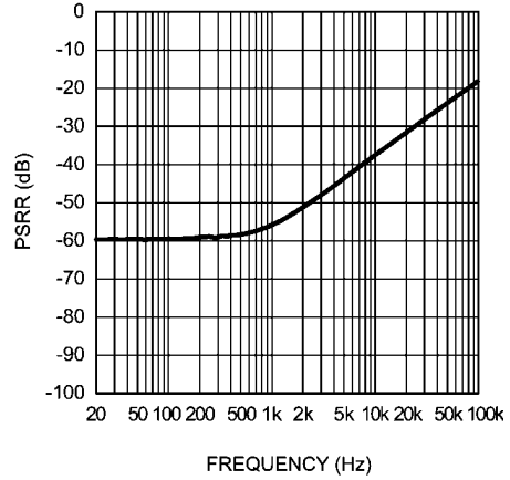
INT/EXT MICBIAS PSRR vs Frequency V_{DD} = 5V , MICBIAS = 2.0V
