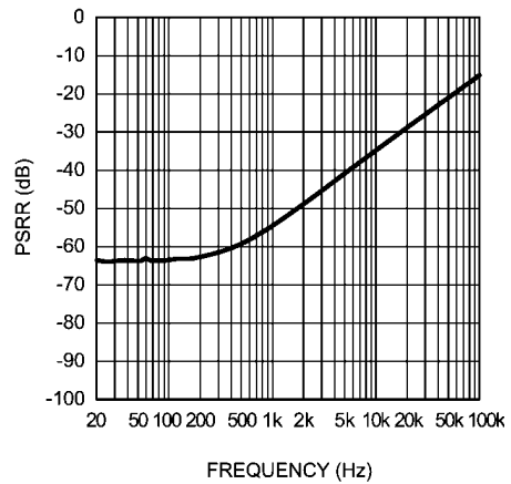
INT/EXT MICBIAS PSRR vs Frequency V_{DD} = 5V , MICBIAS = 2.8V
