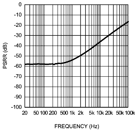
INT/EXT MICBIAS PSRR vs Frequency V_{DD} = 3.3V , MICBIAS = 2.8V
