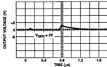
7F. V_{OUT} vs TIME
