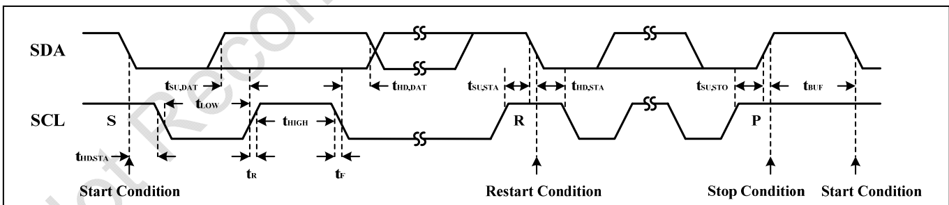
Figure 2 Interface timing
