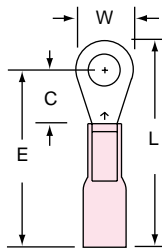
MH18-8R/L Stud Size 8 Wire Range 22-18
