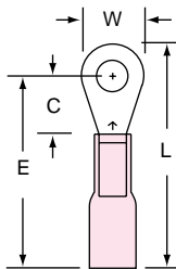
MH18-6R/L Stud Size 6 Wire Range 22-18
