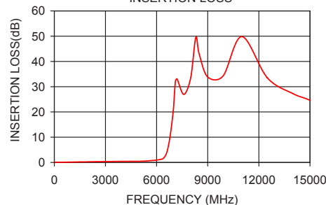
VLF-5850+ INSERTION LOSS
