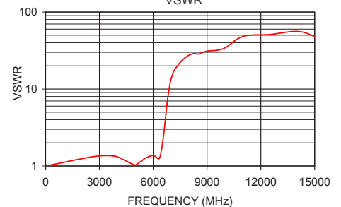
VLF-5850+ VSWR
