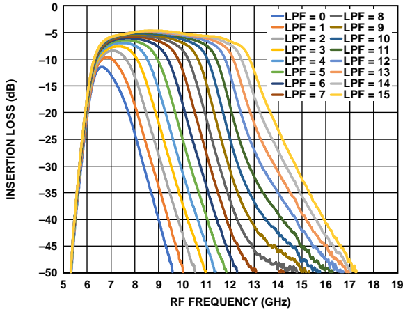
Figure 4. Insertion Loss vs. RF Frequency for HPF State = 0 and LPF State = Swept
