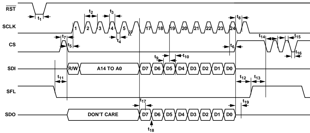
Figure 2. Timing Diagram
