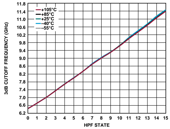
Figure 8. 3 dB Cutoff Frequency vs. HPF State with LPF State = 15 for Various Temperatures
