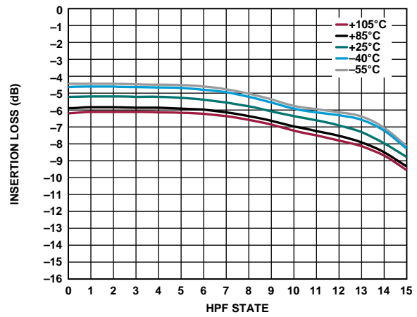
Figure 9. Insertion Loss vs. HPF State with LPF State = 15 for Various Temperatures
