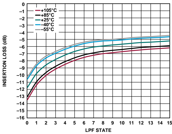
Figure 6. Insertion Loss vs. LPF State with HPF State = 0 for Various Temperatures
