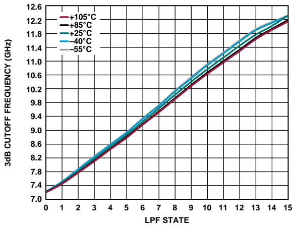
Figure 5. 3 dB Cutoff Frequency vs. LPF State with HPF State = 0 for Various Temperatures
