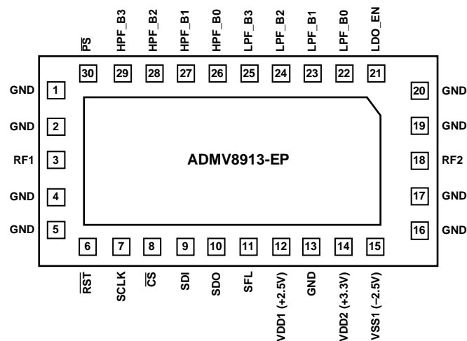
Figure 3. Pin Configuration
