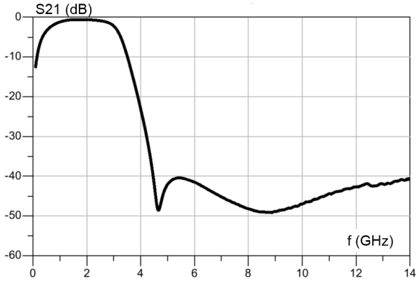
Figure 1. Transmission (dB)
