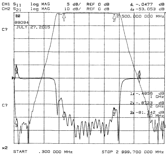
Response Plot:
