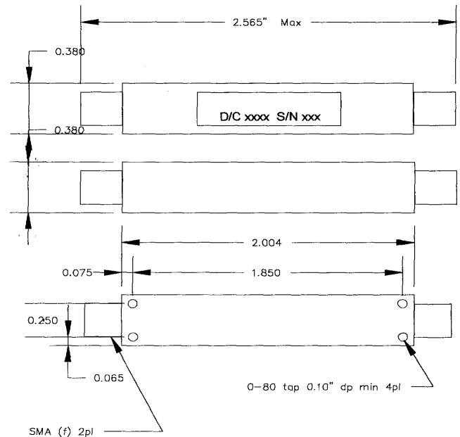
Outline Drawing:
