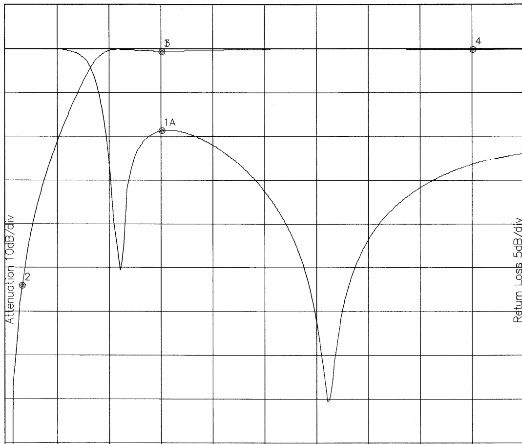
Attenuation/Return Loss
