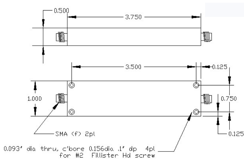
Outline Drawing 986187
