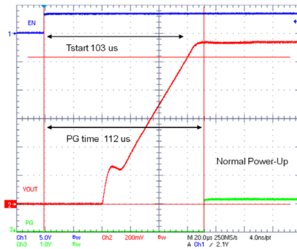
Figure 26. Normal Power Up, V_{\text{OUT}} = 1.15\text{ V}
