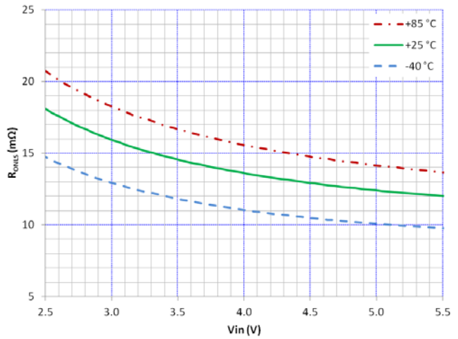
Figure 17. LSS R_{\text{ON}} vs V_{\text{IN}} and Temperature
