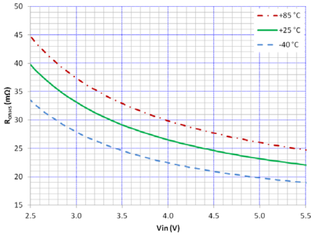
Figure 16. HSS R_{\text{ON}} vs V_{\text{IN}} and Temperature
