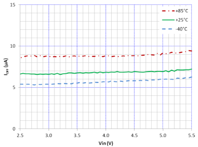
Figure 19. I_{\text{SLEEP}} vs V_{\text{IN}} and Temperature
