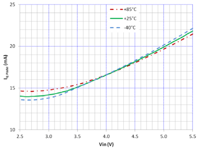
Figure 21. I_{\text{Q PWM}} vs V_{\text{IN}} and Temperature
