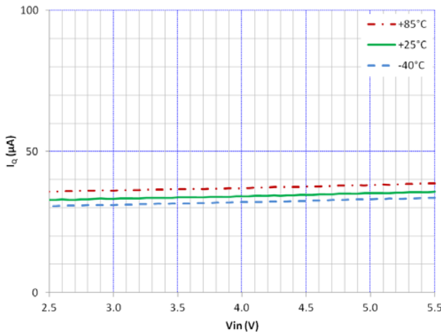
Figure 20. I_{\text{Q PFM}} vs V_{\text{IN}} and Temperature
