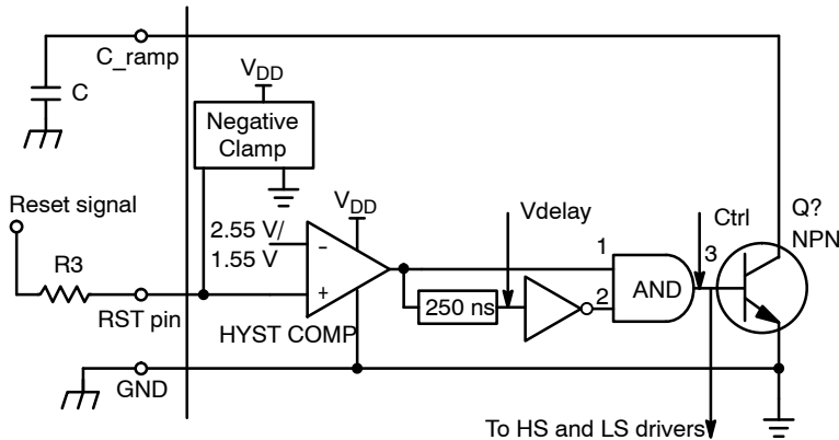
Figure 27. Reset Block
