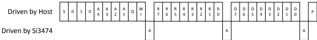
Figure 2.9. 8-Bit Write
