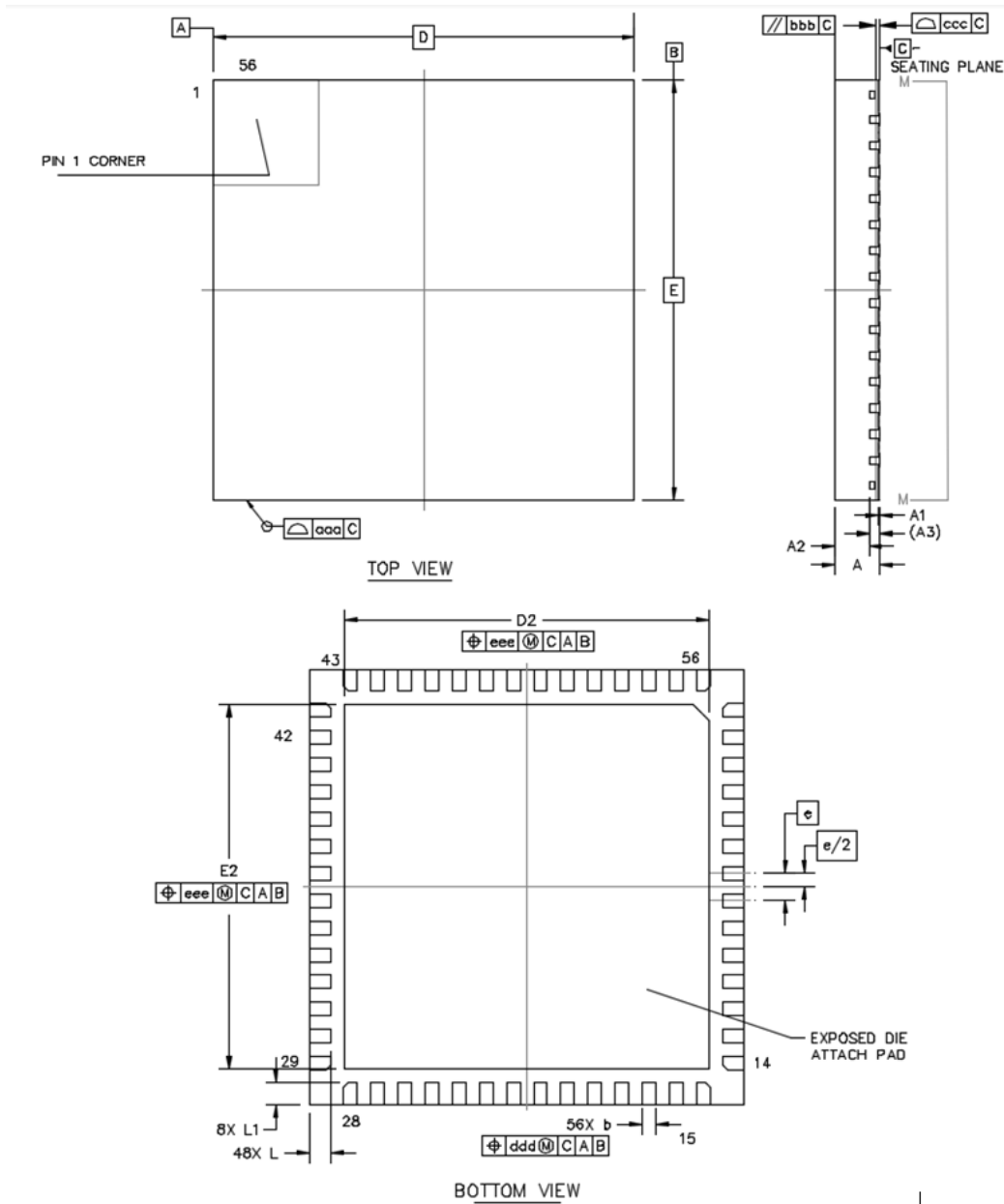
Figure 6.1. 56-Pin QFN Package
