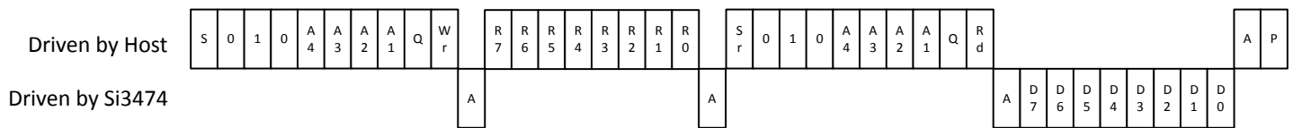
Figure 2.10. 8-Bit Read
