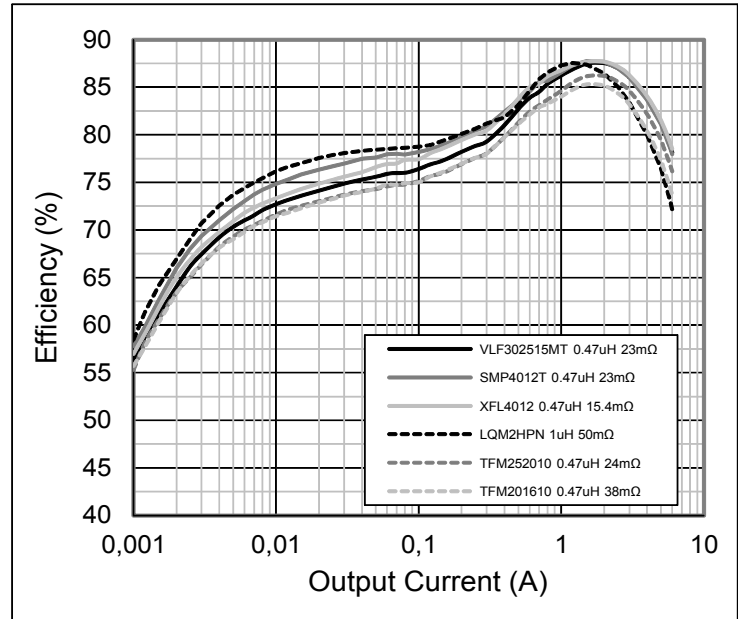
Figure 10: 3.7V Efficiency vs. Output Current Coil Comparison Combined Mode
