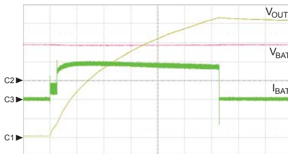
Figure 14. Input current waveforms with Li+ battery connected through 4.7 \mu H inductor and 10 \mu F capacitor, C_{OUT} = 100 \mu F, V_{IN} = V_{BAT} = 3.6 V, Ch1: V_{OUT} = 50 V/div, Ch2: V_{BAT} = 2 V/div, Ch3: I_{BAT} = 200 mA/div, t = 1 s/div
