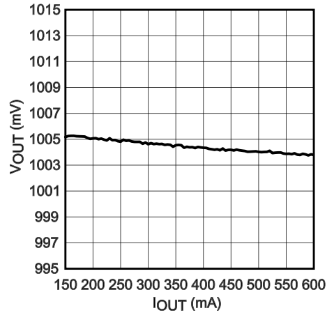
Buck 3 V_{OUT} vs. I_{OUT} V_{IN}=5.0V, V_{OUT}=1.0V
