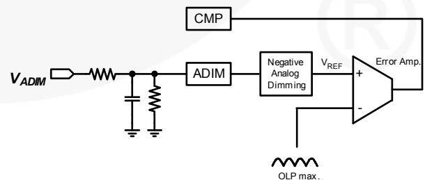
Figure 38. Analog Implementation Circuit
