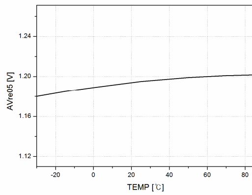
Figure 18. Analog Dimming Reference Voltage 05 vs. Temperature
