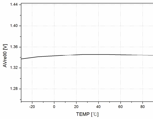
Figure 17. Analog Dimming Reference Voltage 00 vs. Temperature
