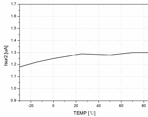
Figure 20. Error Amplifier Source Current 2 vs. Temperature
