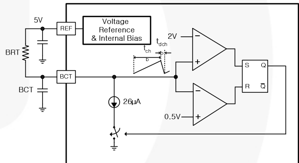
Figure 37. Burst Dimming Oscillator Circuit
