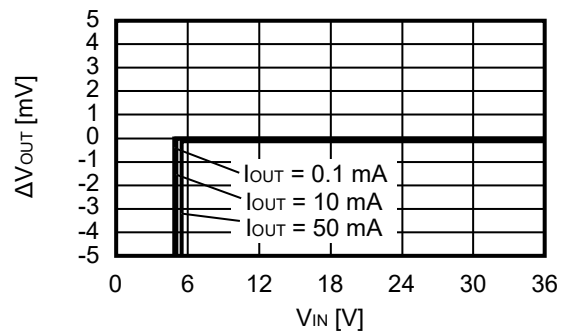
8.1 V_{ADJ/EN} = 5.0\text{ V}
