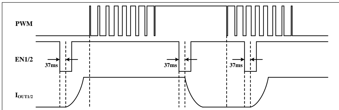
Figure 61 Priority Logic 2 of EN1/2 in Low Pulse Mode
