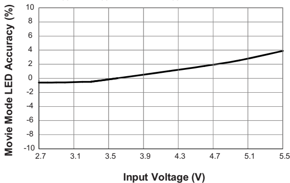
Movie Mode Current Accuracy vs. Input Voltage
