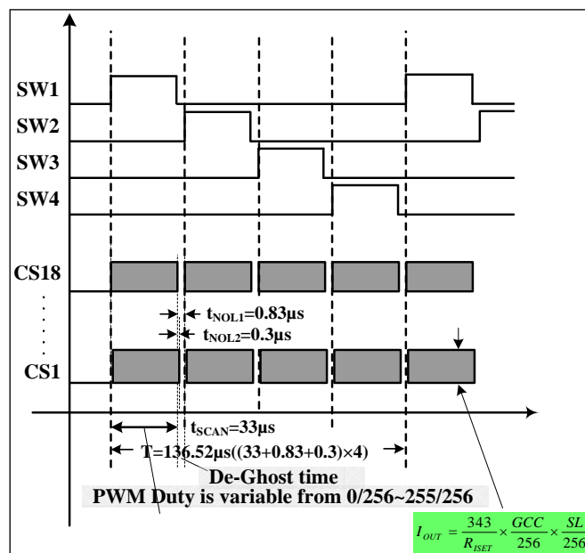
Figure 6 Scanning Timing
