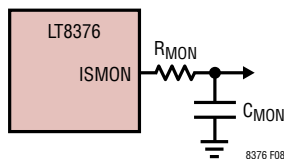
Figure 8. Resistor Configuration
