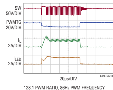
128:1 PWM RATIO, 86Hz PWM FREQUENCY
