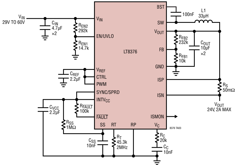
24V Voltage Regulator with Spread Spectrum
