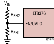
Figure 13. EN/UVLO Resistor Configuration
