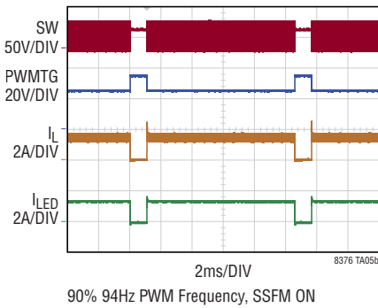
Internal PWM Dimming
