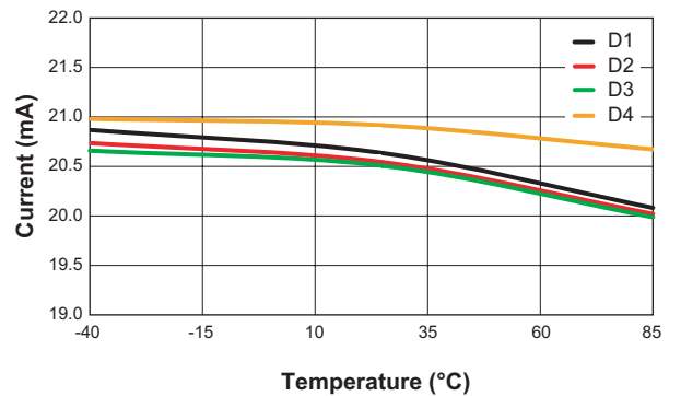
AAT3195-2 Current Matching vs. Temperature
