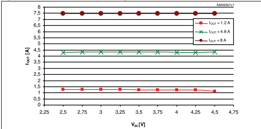
Figure 16. Torch current vs. input voltage
