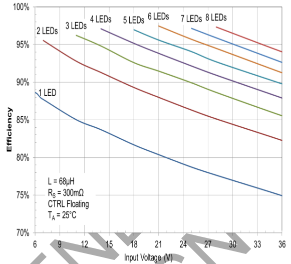
Figure 14 Efficiency vs. Input Voltage
