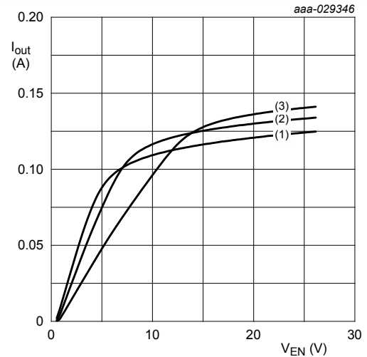
Fig. 9. NCR420U: Output current as a function of enable voltage; typical values
