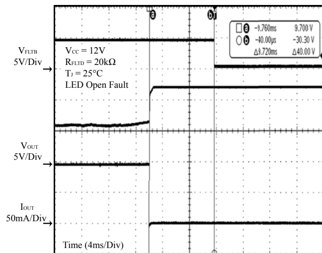
Figure 33 t_{FLT}
