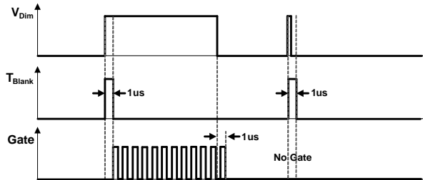
Figure 20. PWM Dimming
