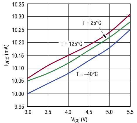
I VCC vs V CC – Channel On, Data Off
