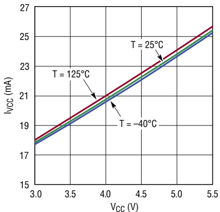
I VCC vs V CC – Channel On, Data On
